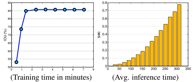
Figure 5: Time: (Left) IOU as a function of training time, (Right) average inference time as a function of scale.
